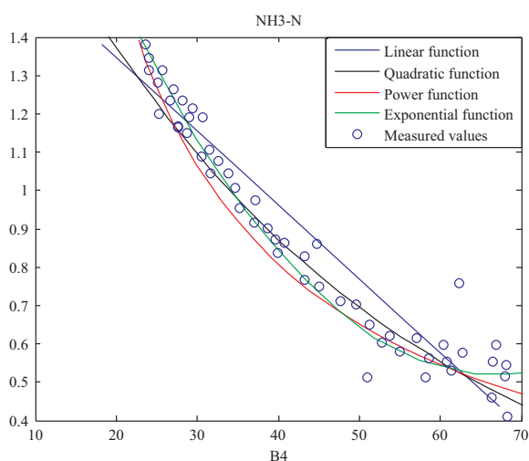
Fig. 9. The estimation model between NH 3 -N and B 4 .
