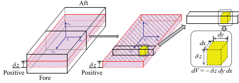
Fig. 4. Infinitesimal volume for floating structures in immersion.
