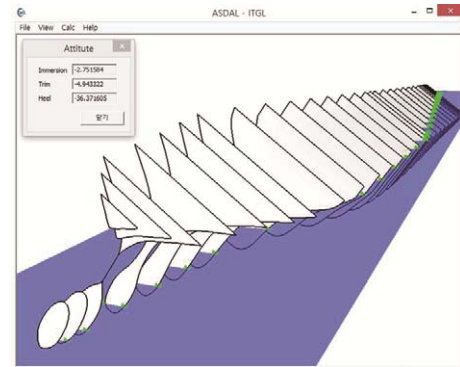
Fig. 12. The position and attitude of the 4800TEU Container Carrier in static equilibrium state.
