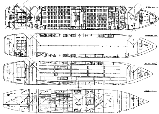
Fig. 3. The layout of every deck.
