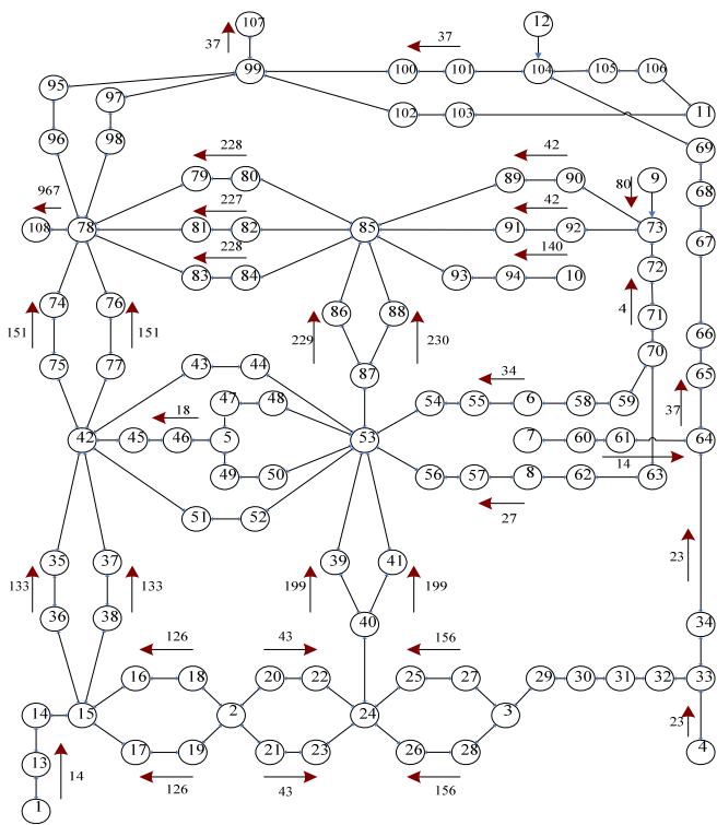
Fig. 6. Proposed evacuation route of "TAI WHA" based on our model.
