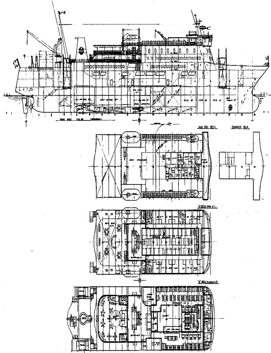
Fig. 2. The Ro-Ro passenger ferry, “TAI WHA”.
