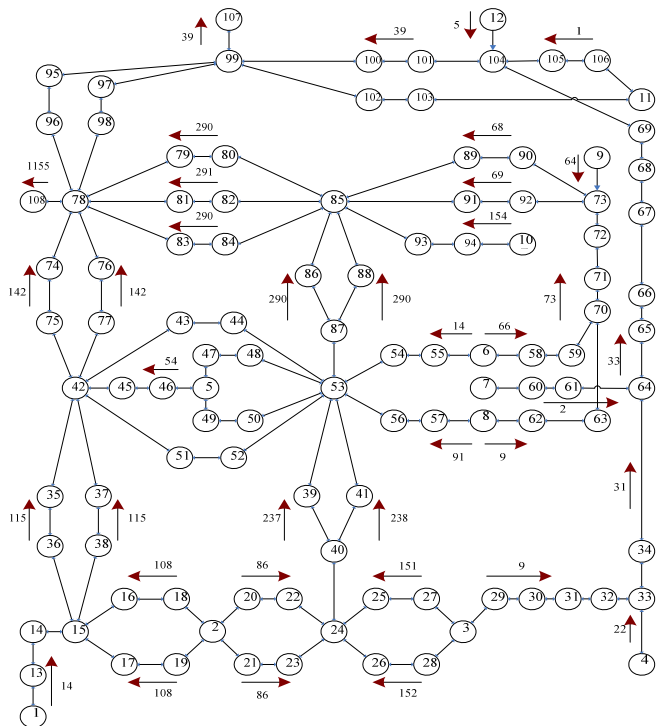
Fig. 7. Proposed evacuation route based on the moderate condition.
