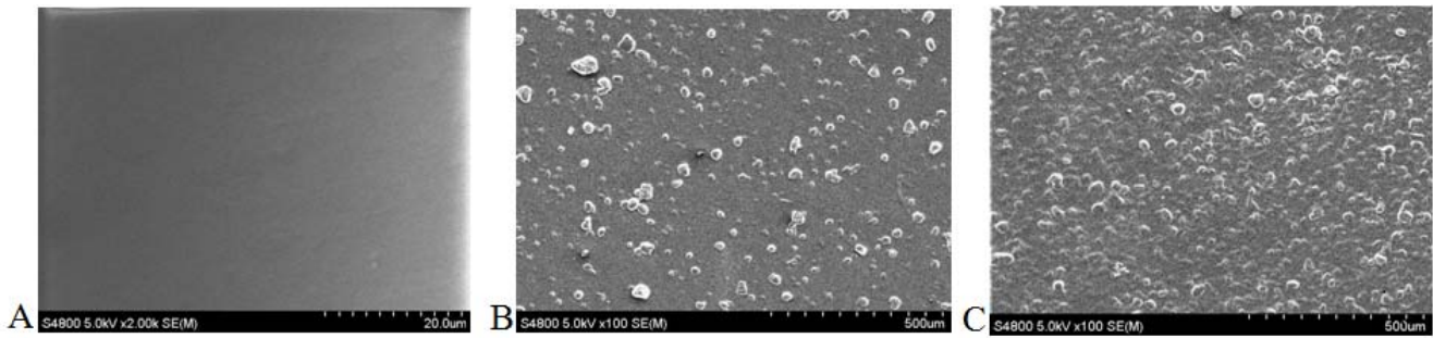
Fig. 2 SEM micrographs of CS/GEL/FHAP membrane before (B) and after (C) sintering. The CS/GEL membrane (as a control) is shown in the image (A).
